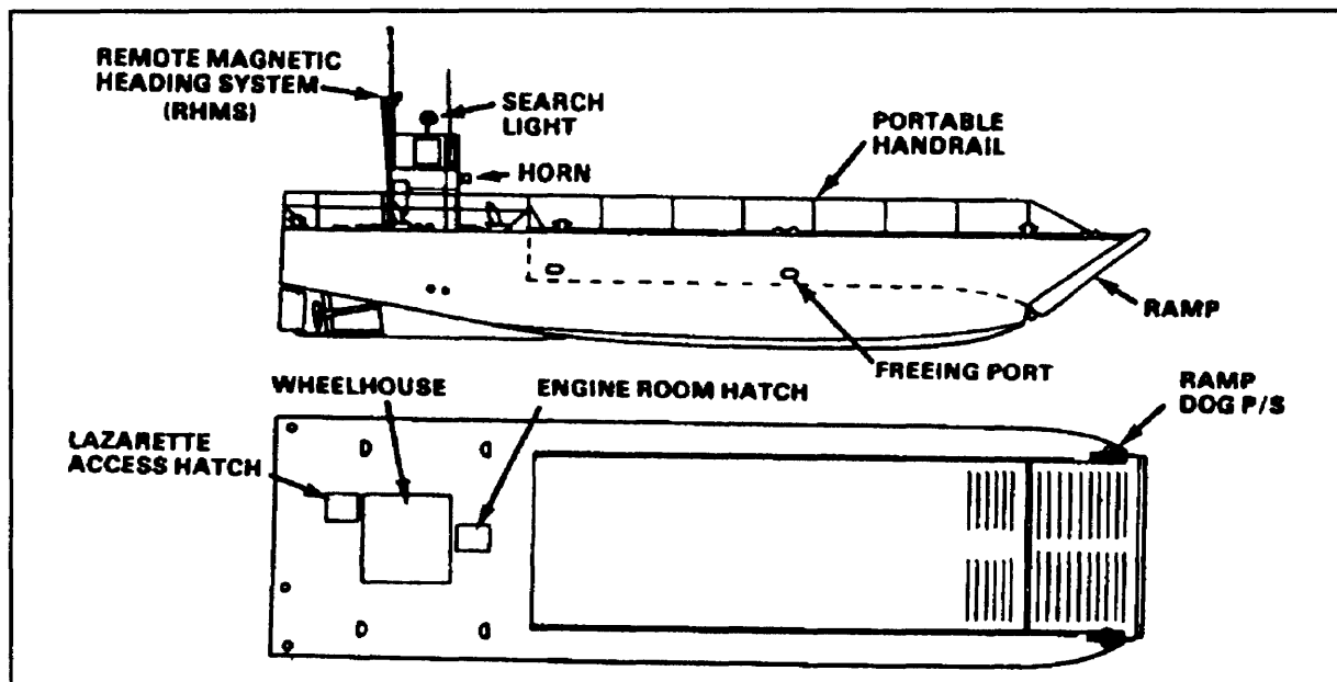
Figure 2-3. Landing Craft, Mechanized (LCM-8).
