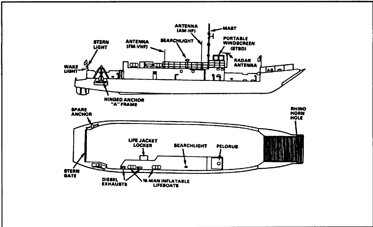
Figure 2-5. Landing Craft, Utility (LCU), 1600 Class.
