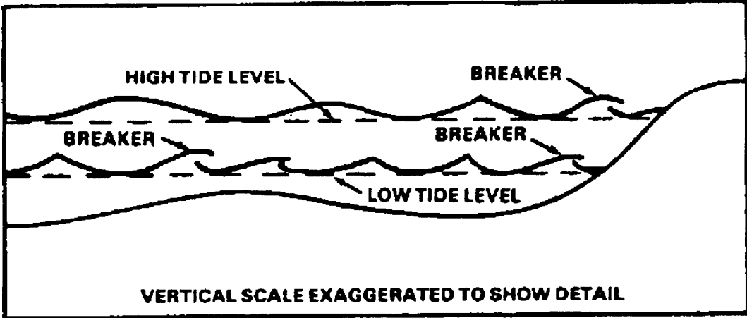
Figure 11-3. Effect of Tide on Surf Zone.
